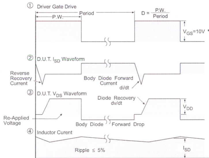
Fig 14. For N-Channel HEXFET® MOSFETs
